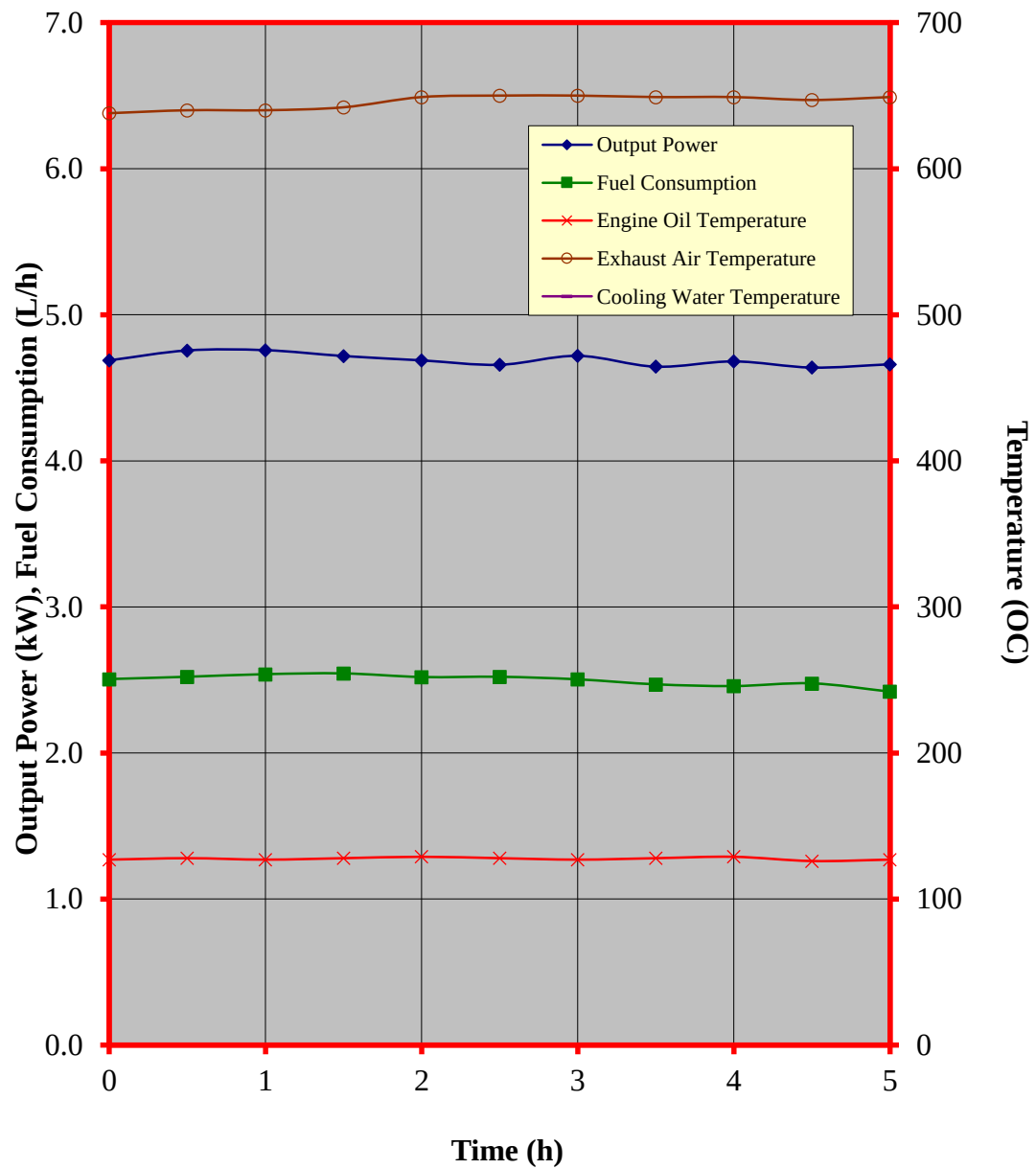
Figure 4. Performance characteristic curves during the continuous running test of the HONDA GX270H QP gasoline engine
