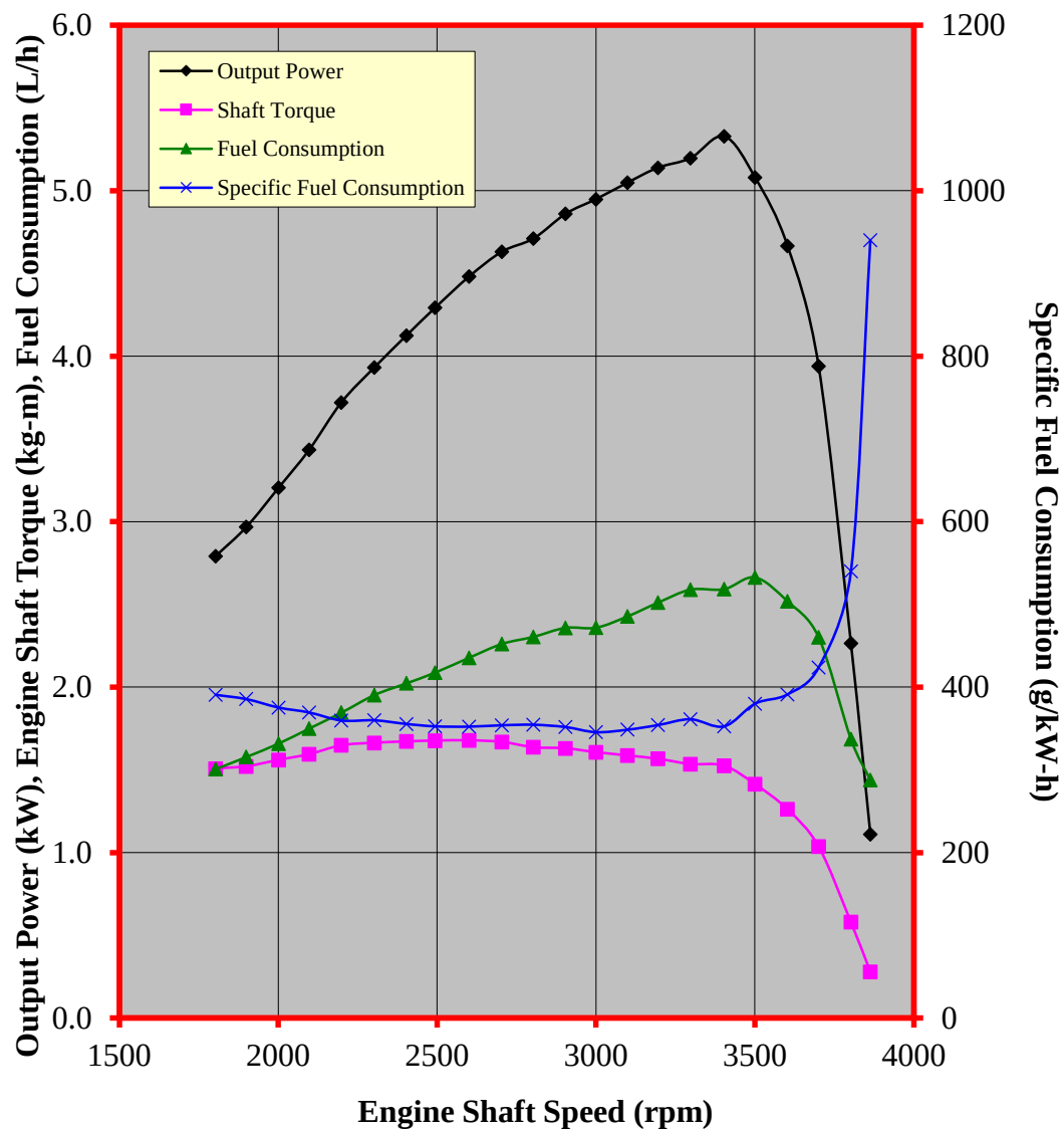
Figure 3. Performance characteristic curves of the HONDA GX270H QP gasoline engine
